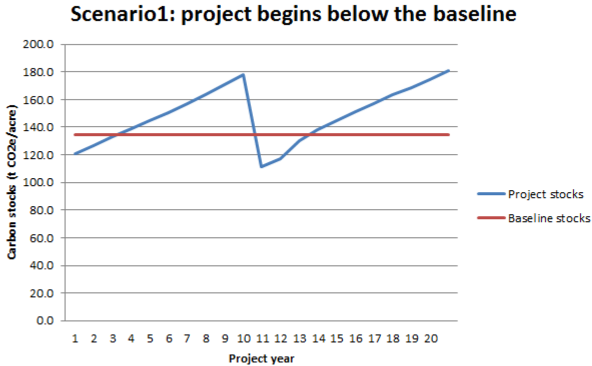
Addendum Figure 1. Illustration of baseline and project dynamics when project stocks begin below the baseline
